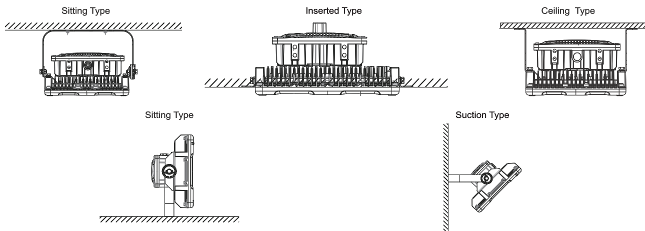
Installation Mode
